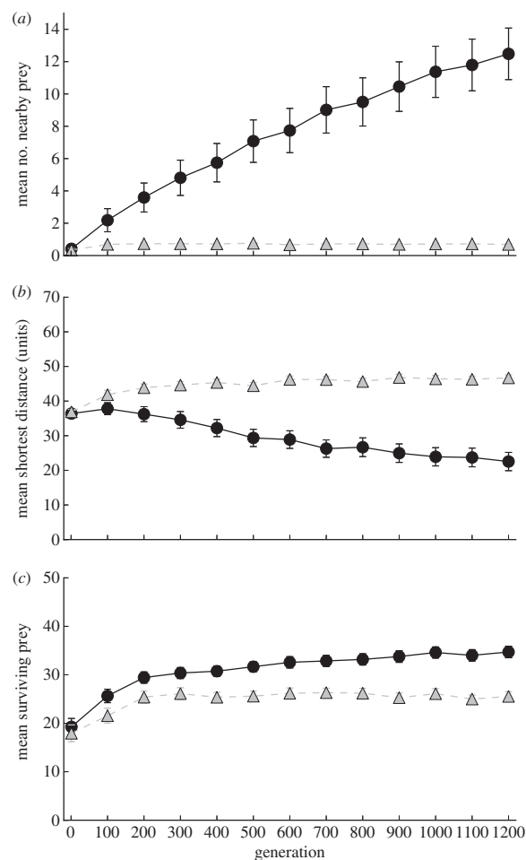
Figure 4. Mean swarm density ( a ), swarm dispersion ( b ) and survivorship ( c ) within the swarm over all replicates over evolutionary time. The swarm density was measured by the mean number of prey within 30 virtual metres of each other over a lifespan of 2000 simulation time steps. Swarm dispersion was measured by the mean distance to the nearest prey for every living prey over a lifespan of 2000 simulation time steps. Survivorship within the swarm was measured as the mean number of surviving prey (out of an initial total of 50) at the end of the simulation at a given generation. Prey hunted by a predator with predator confusion (black circles with a full line) evolved to maintain significantly higher swarm density and significantly less dispersed swarming behaviour than prey in the swarms hunted by a predator without predator confusion (grey triangles with a dashed line). As a result, significantly more prey survived in the swarms hunted by a predator with predator confusion than the swarms hunted by a predator without predator confusion. Error bars indicate 2 s.e. across 180 replicate experiments.
