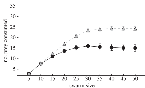
Figure 6. Functional response curves of cohesive swarms hunted by a predator with predator confusion (black circles with a full line) and dispersed swarms hunted by a predator without predator confusion (grey triangles with a dashed line). The evolved, cohesive swarms hunted by a predator with predator confusion result in a type II functional response with a lowered plateau. Error bars indicate 2 s.e. across 180 replicate experiments.
