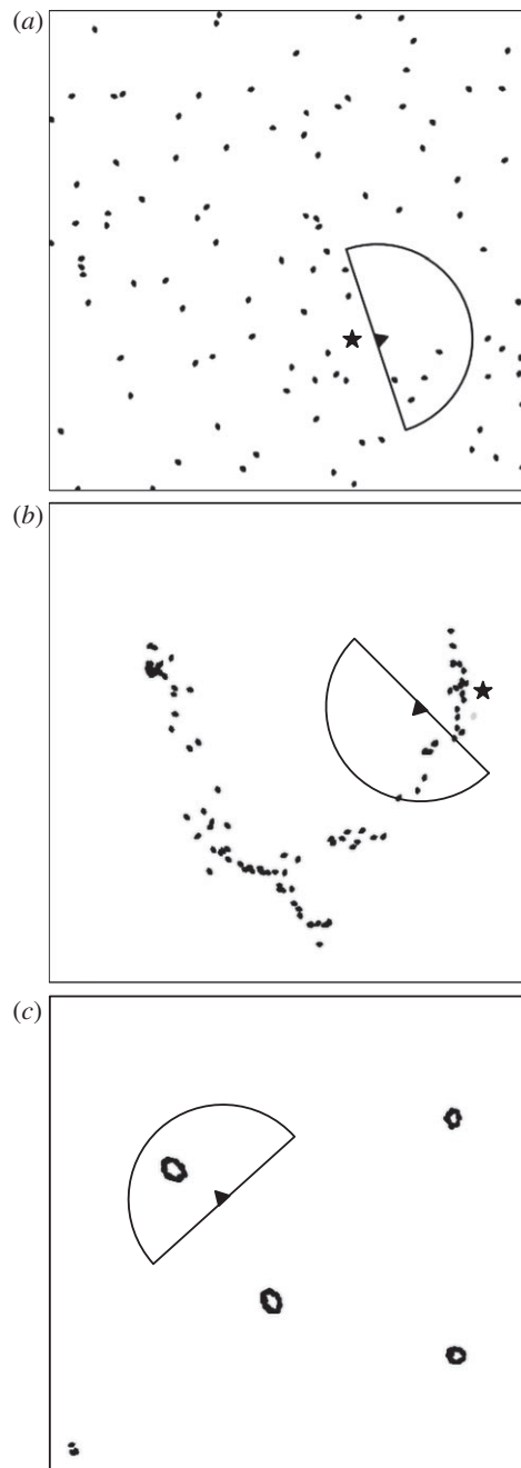
Figure 3. Screen captures of (a) dispersed prey in a swarm hunted by a predator without predator confusion, (b) prey forming a single elongated swarm under attack by a predator with predator confusion and (c) prey forming multiple cohesive swarms to defend themselves from a predator with predator confusion after 1200 generations of evolution. Black dots are prey, the triangle is the predator, the lines projecting from the predator represent the predator's frontal 180° visual field, and the star denotes where a prey was just captured.
